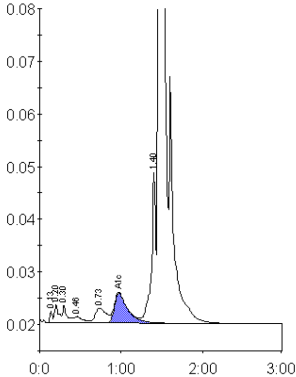
Peak table - ID: 10512286
